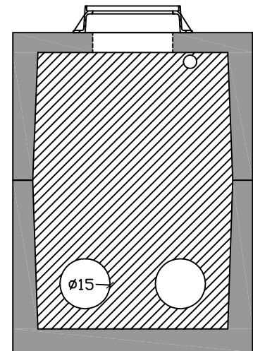
Baffle View
