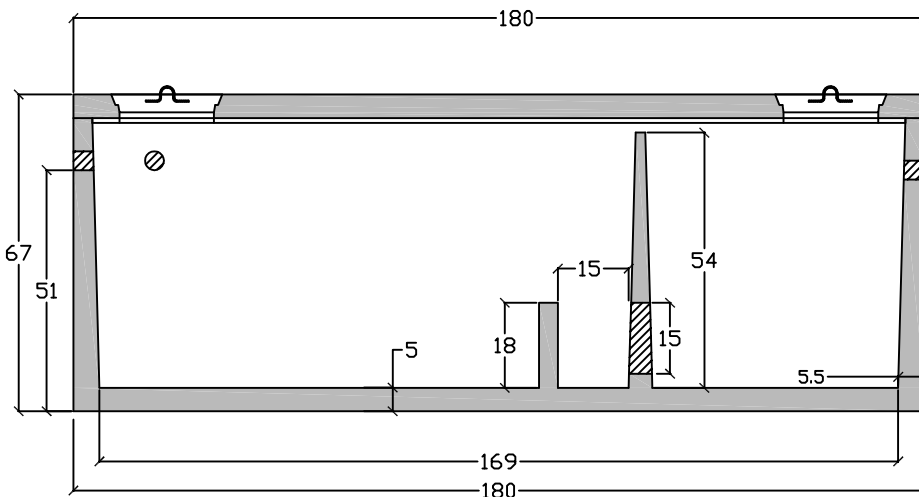
Side View
