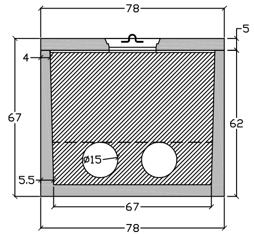
Baffle View
