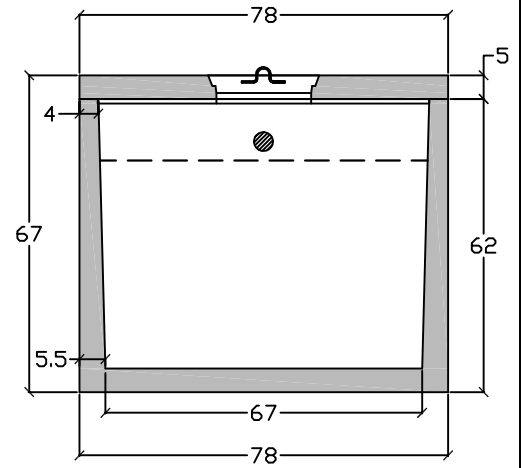
End View
