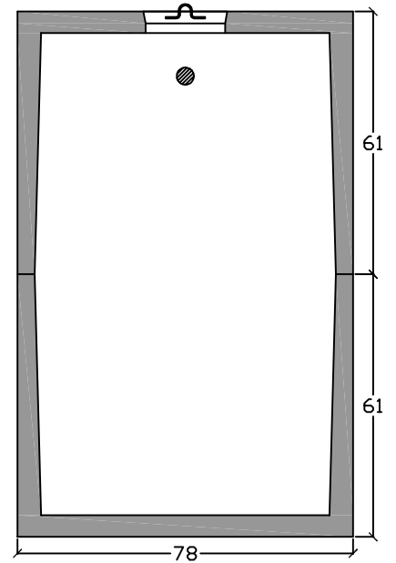
End View
