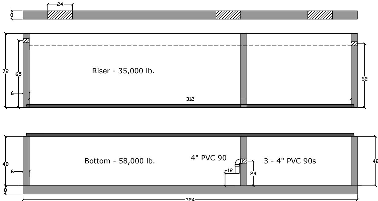
Side View
