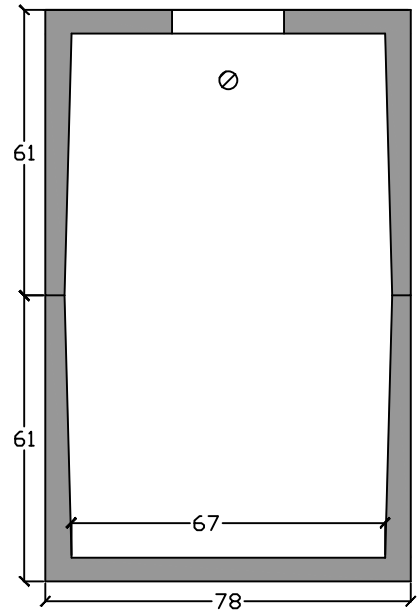
End View
