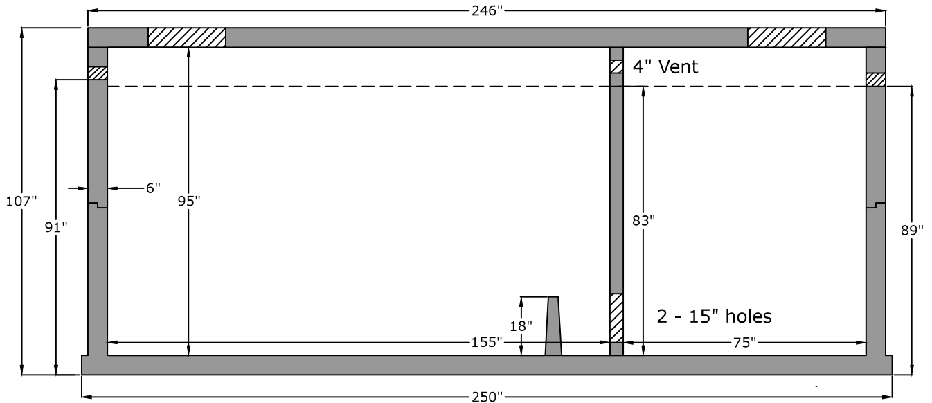
Side View
