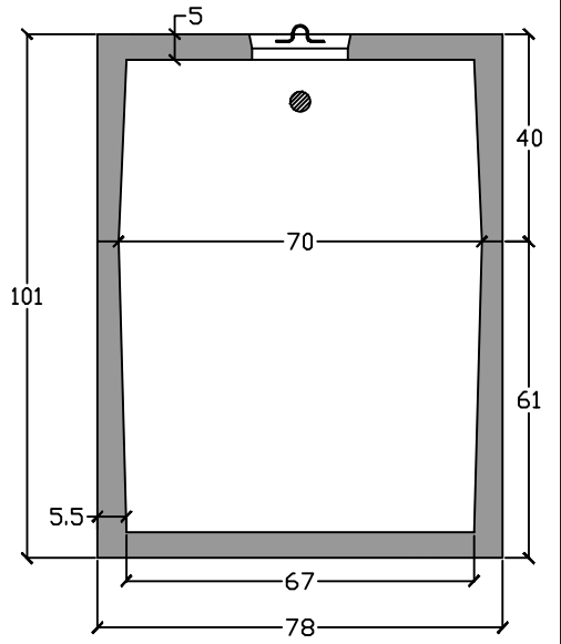
End View
