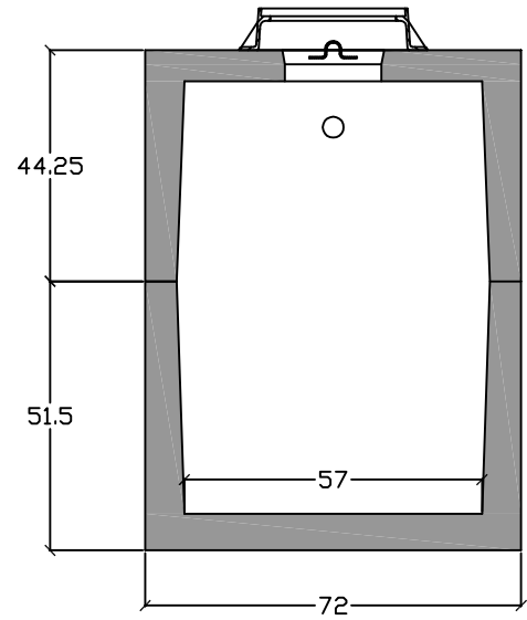
End View
