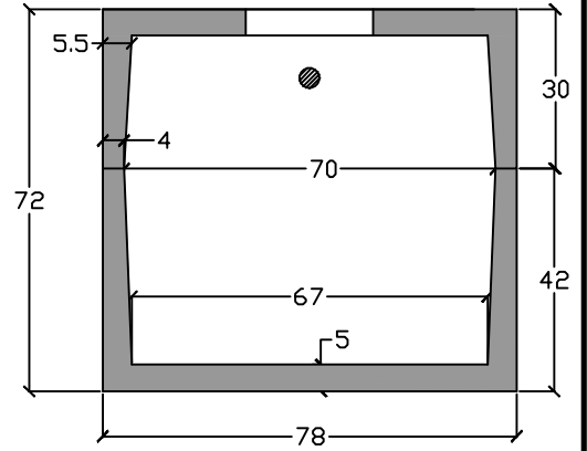
End View
