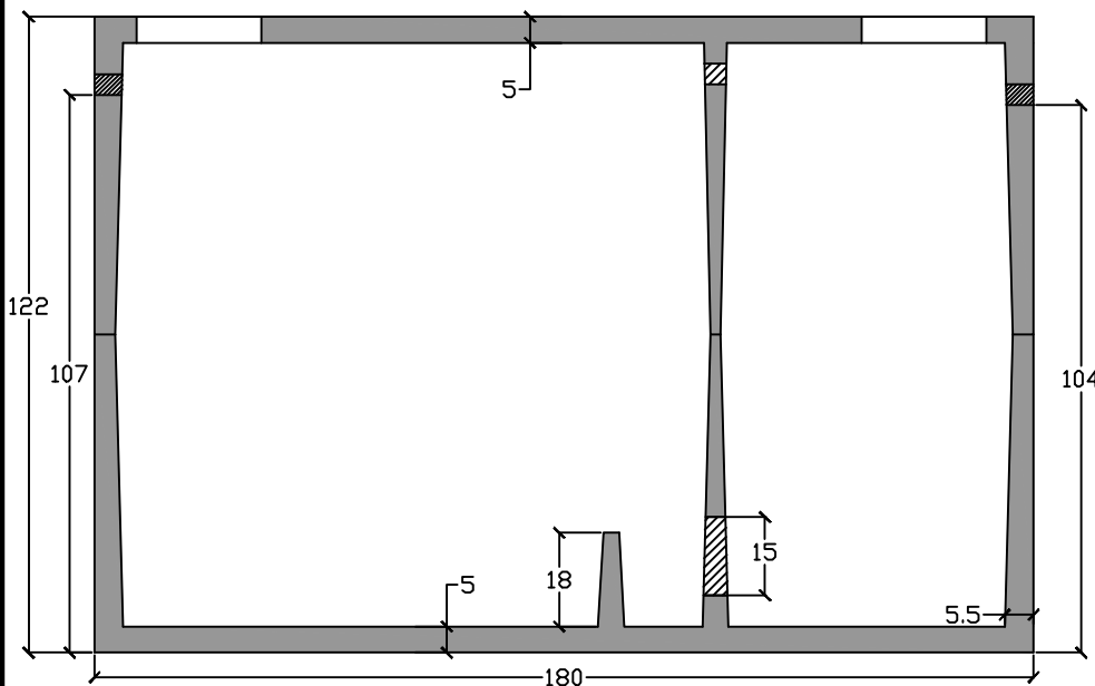
Side View
