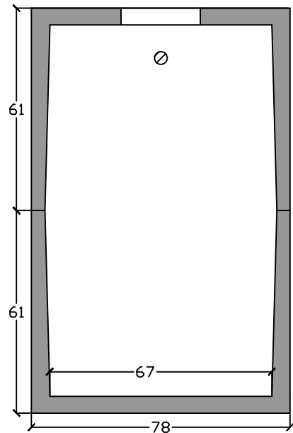
End View
