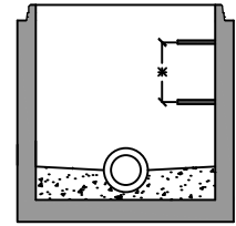
Manhole Base Preformed Invert Detail
