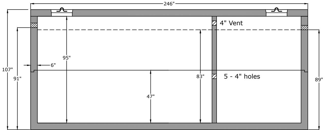
Side View
