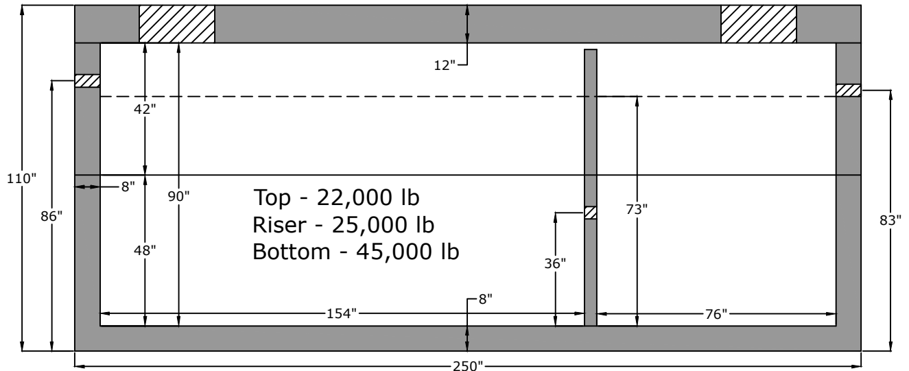
Side View
